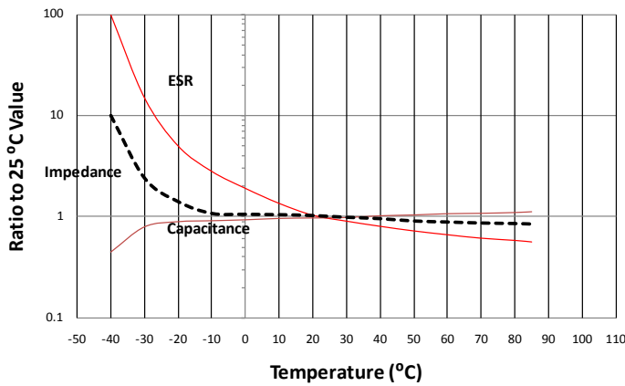
Temperature Characteristics - 29,000 \mu F 50 Vdc
