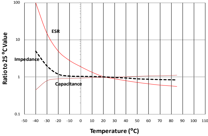
Temperature Characteristics - 4,600 \mu F 100 Vdc
