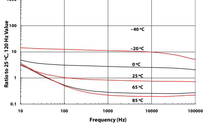
ESR vs Temperature and Frequency, 1300 \mu F 500 V
