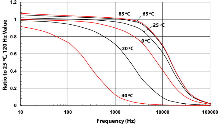
Capacitance vs Temperature and Frequency, 1300 \mu F 500 V
