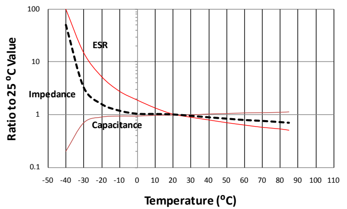
Temperature Characteristics - 100,000 \mu F 10 Vdc
