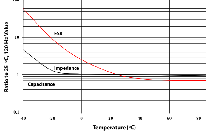
Temperature Characteristics, 4800 \mu F 200 V
